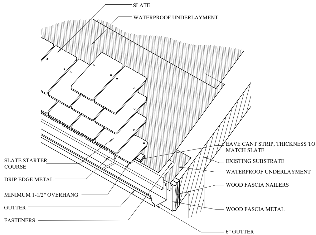
ROOF EDGE WITH GUTTER
