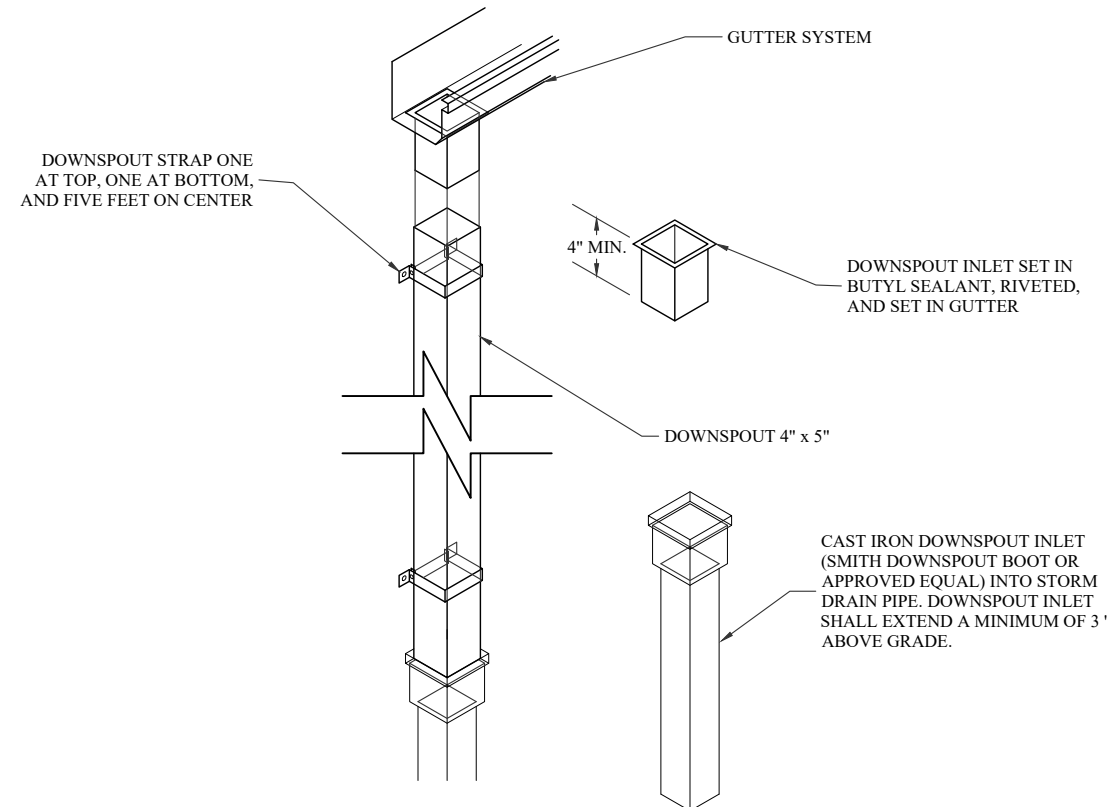
DOWNSPOUT
