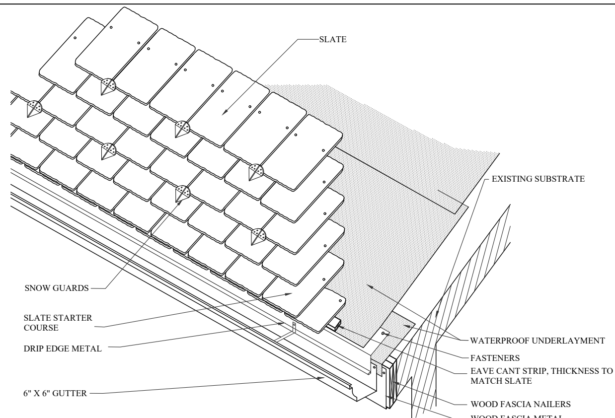
SNOW GUARD PATTERN
