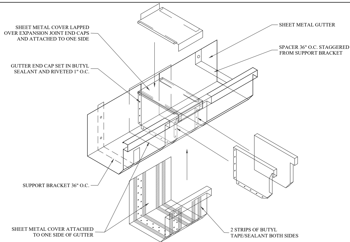
GUTTER EXPANSION JOINT
